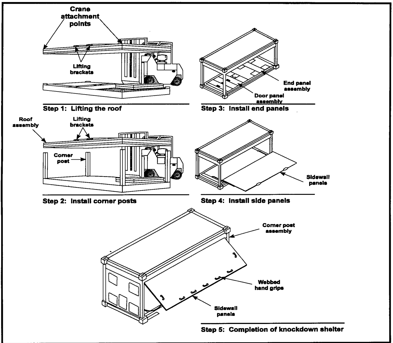
Figure 7-3. MCESS Shelter Assembly Process
