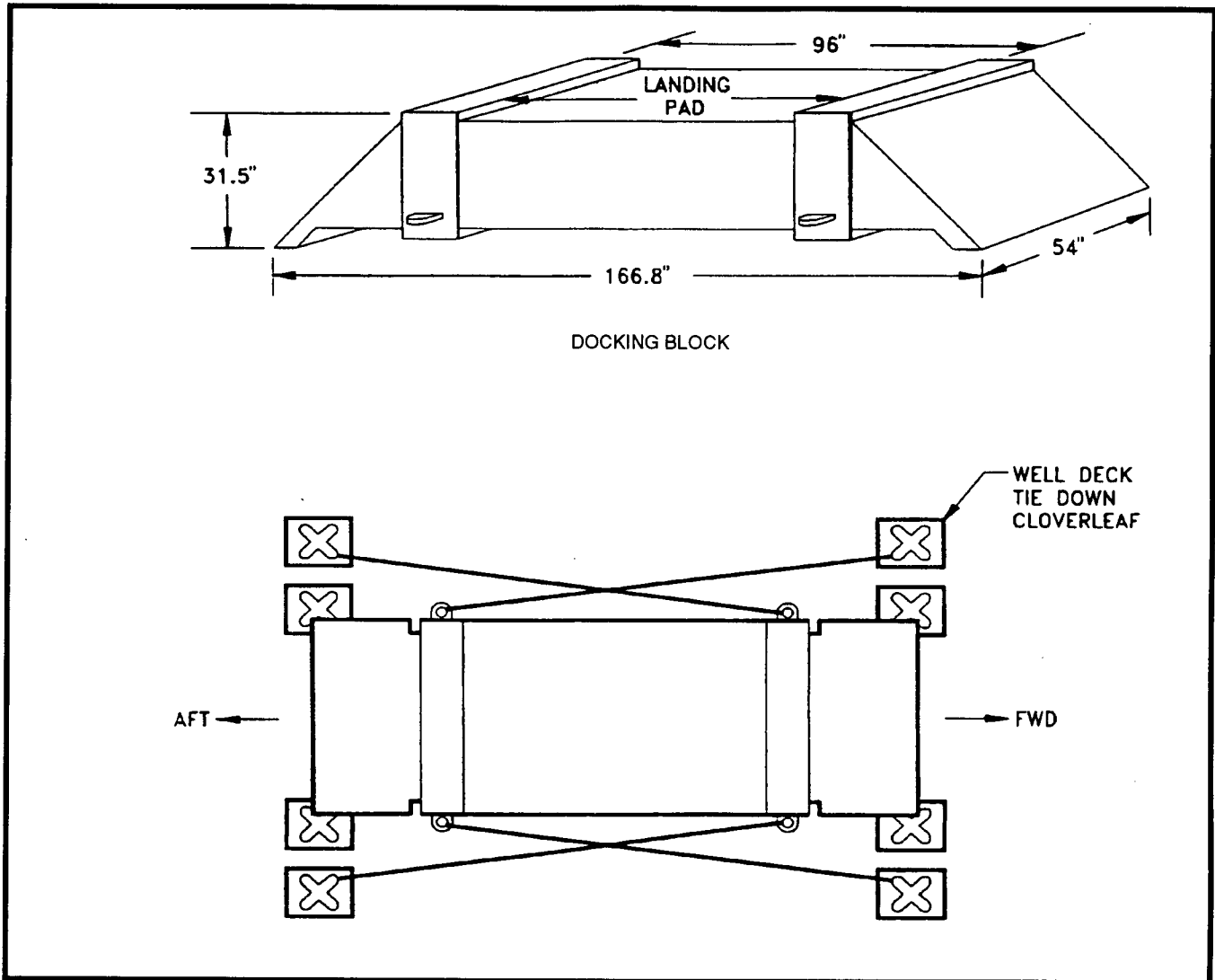
Figure A-5. LCAC Docking Block and a Typical Tiedown Configuration
