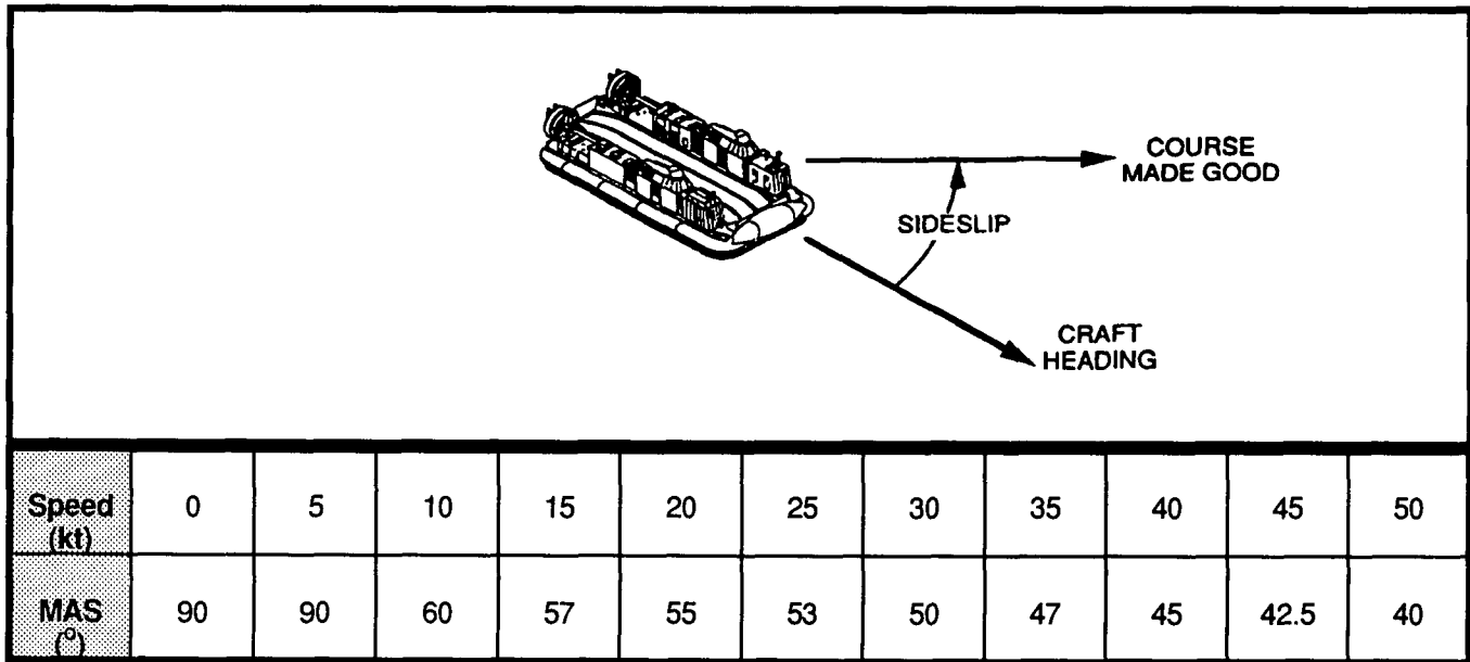
Figure 4-8. Maximum Allowable Slideslip
