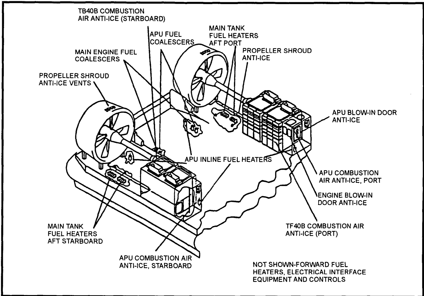
Figure A-3. LCAC Cold Weather Kit Component Location
