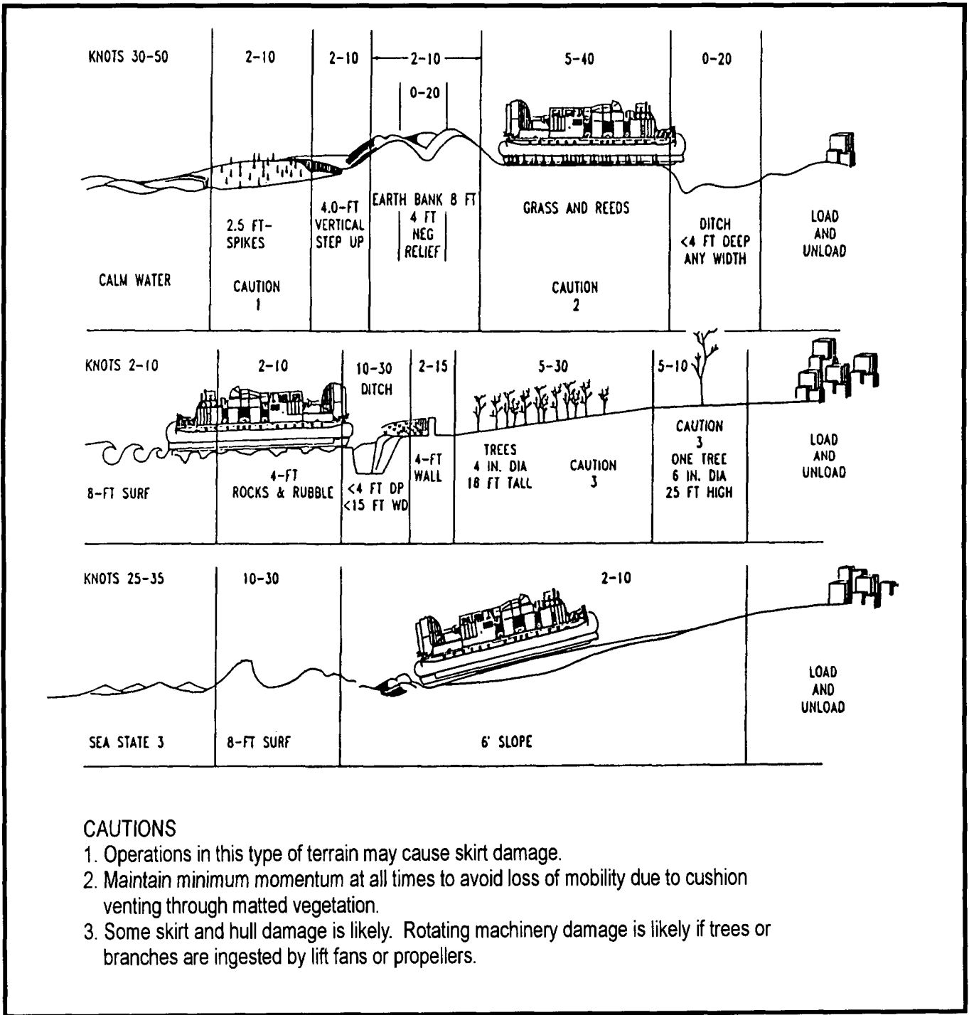
Figure 1-5. Rough Terrain Capabilities
