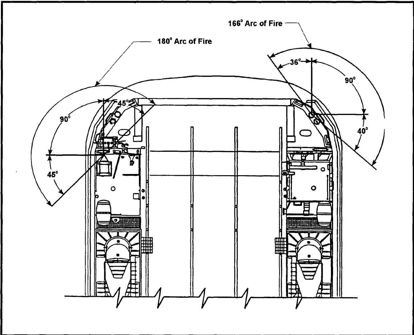
Figure 5-2. LCAC 1 Through 33 Firing Arcs
