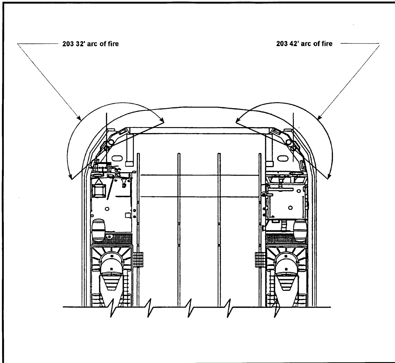
Figure 5-3. LCAC 34 Through 84 Firing Arcs
