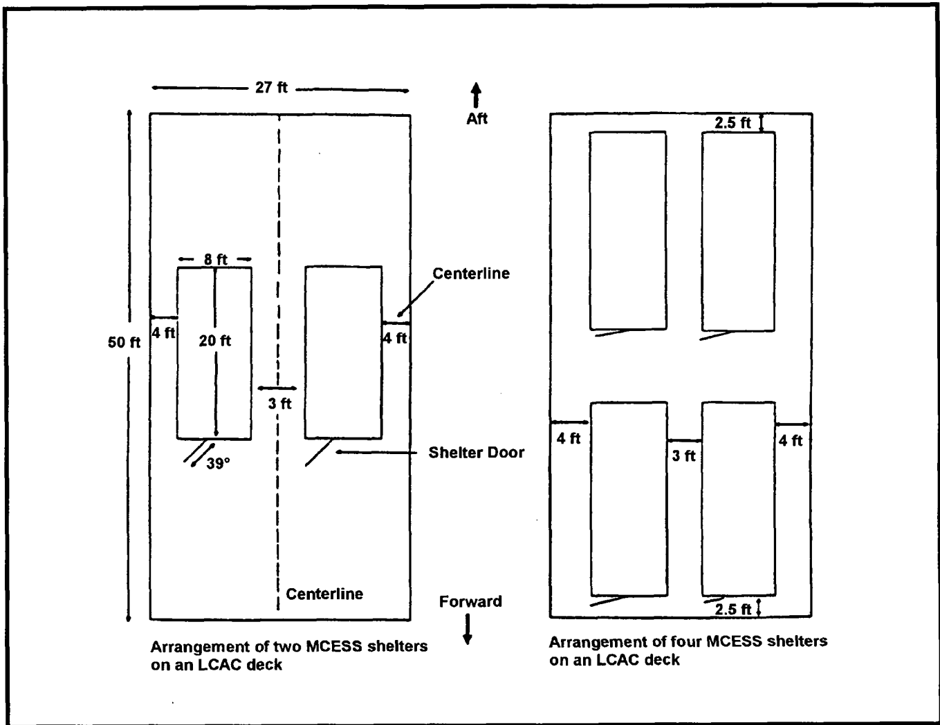
Figure 7-4. MCESS Shelter Configurations (Sheet 1 of 3)
