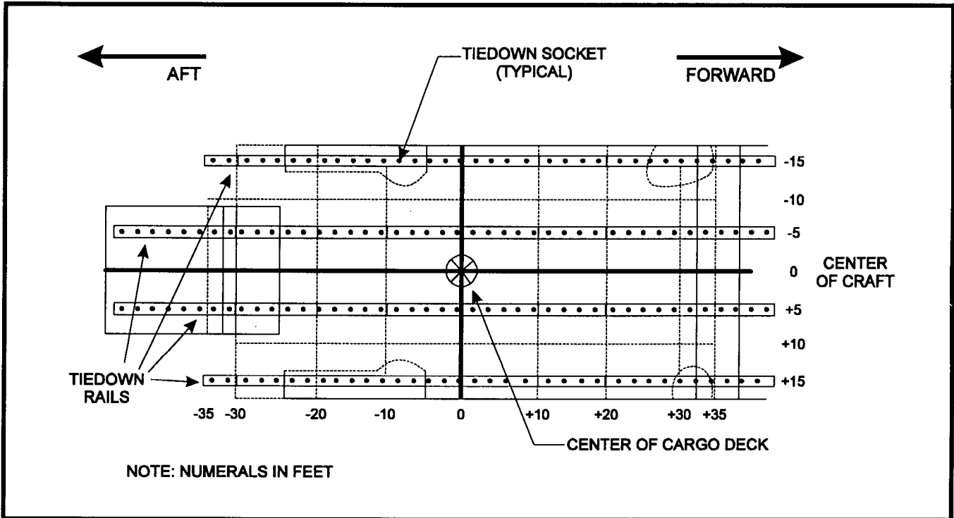
Figure C-2. LCAC Cargo Deck Grid
