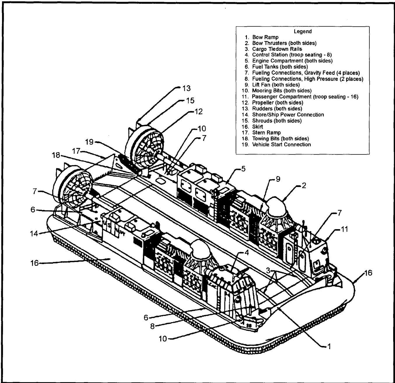
Figure A-1. LCAC Primary Features
