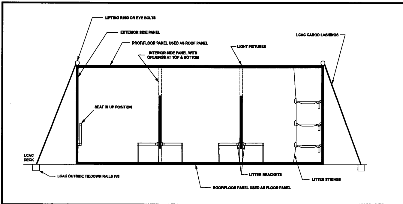
Figure 7-7. LCAC PTM Cross Sectional View
