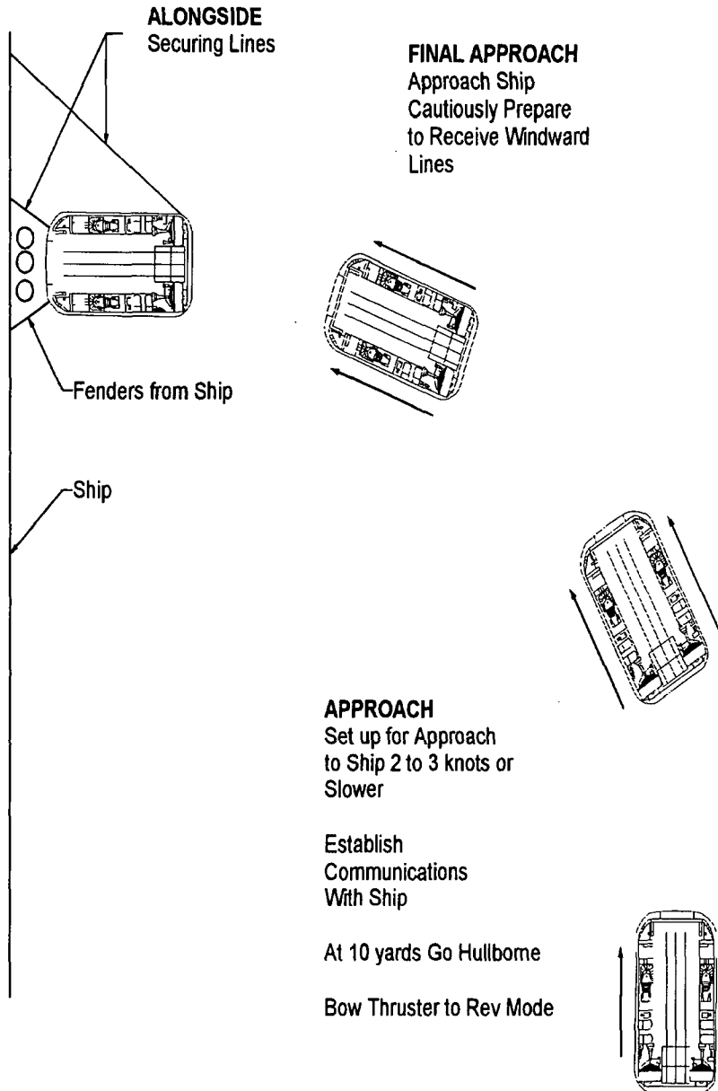
Figure A-8. LCAC Mooring to a Ship
