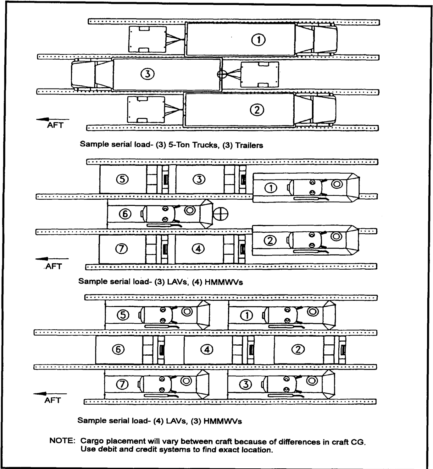
Figure C-7. LCAC Standard Loads and Standard Load Equivalents (Sheet 4 of 4)
