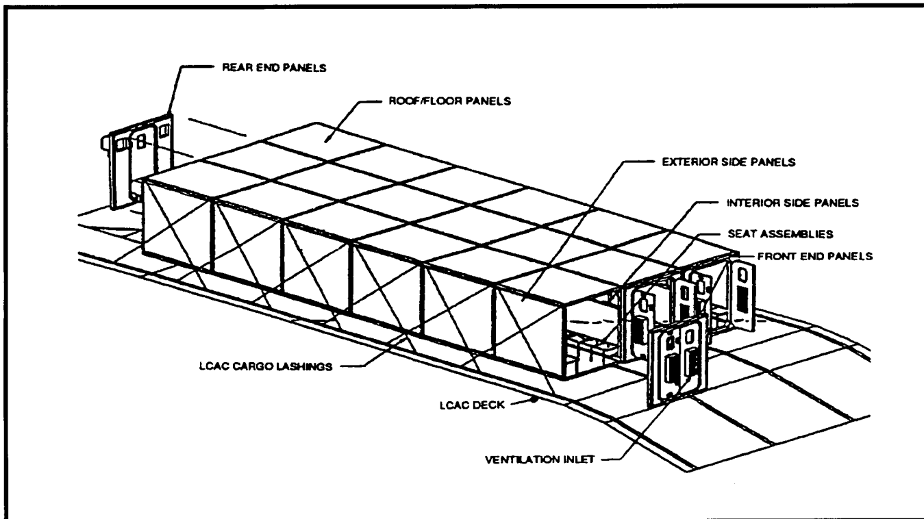
Figure 7-5. Six-Section PTM-Configured LCAC with Major Components
