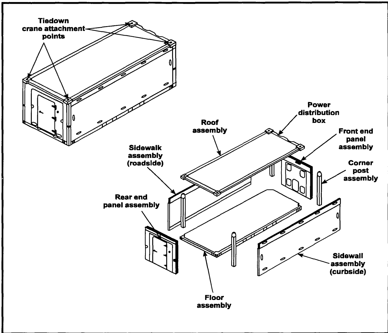
Figure 7-2. Knockdown MCESS Shelter and Major Components
