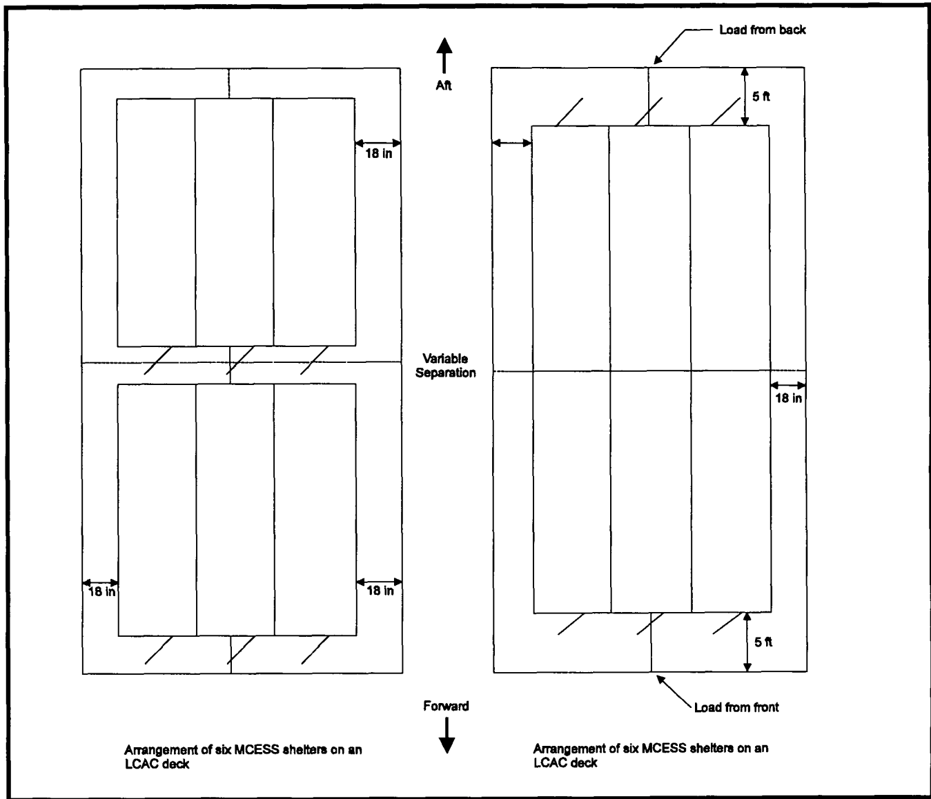
Figure 7-4. MCESS Shelter Configurations (Sheet 3 of 3)
