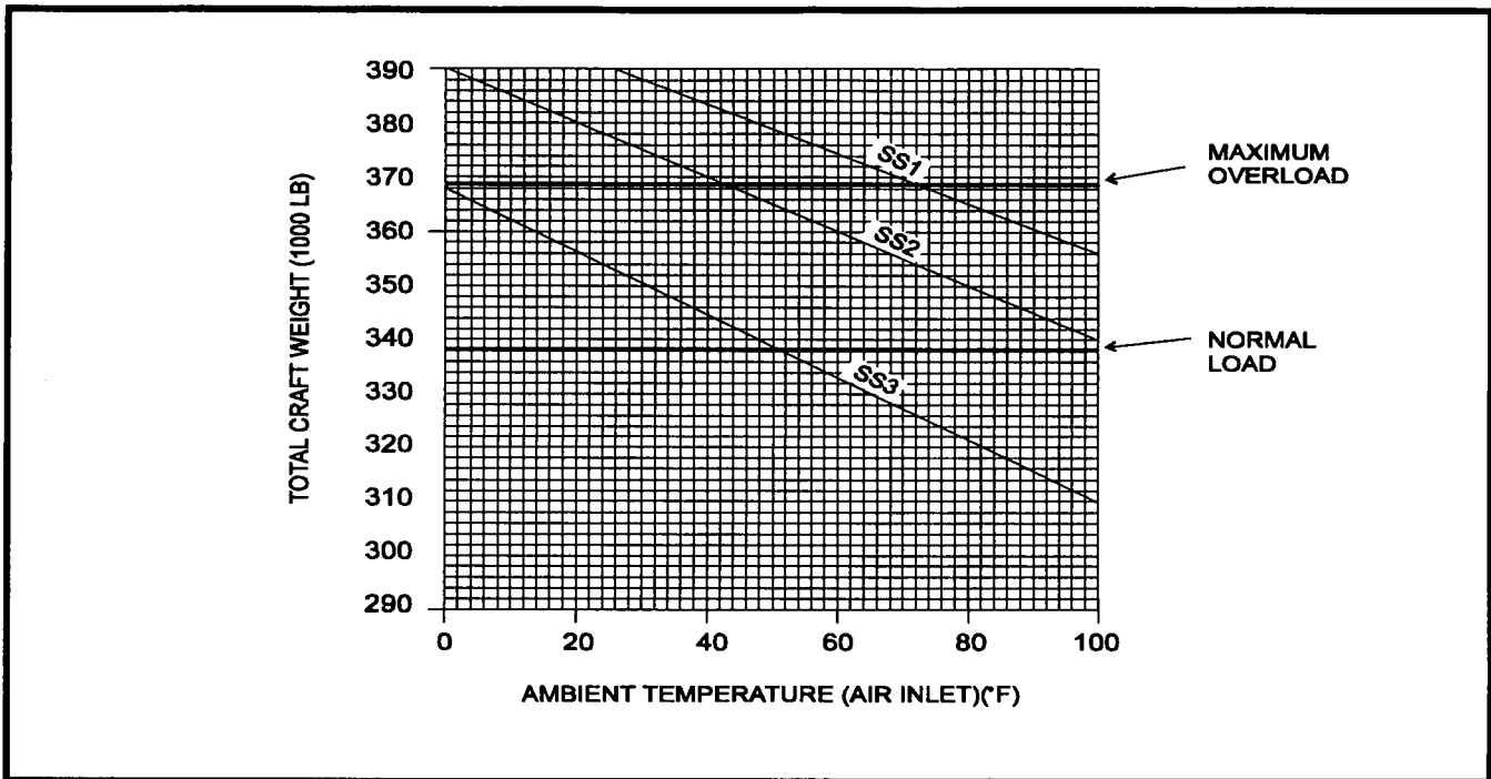
Figure 8-3. LCAC Load as a Function of Ambient Temperature
