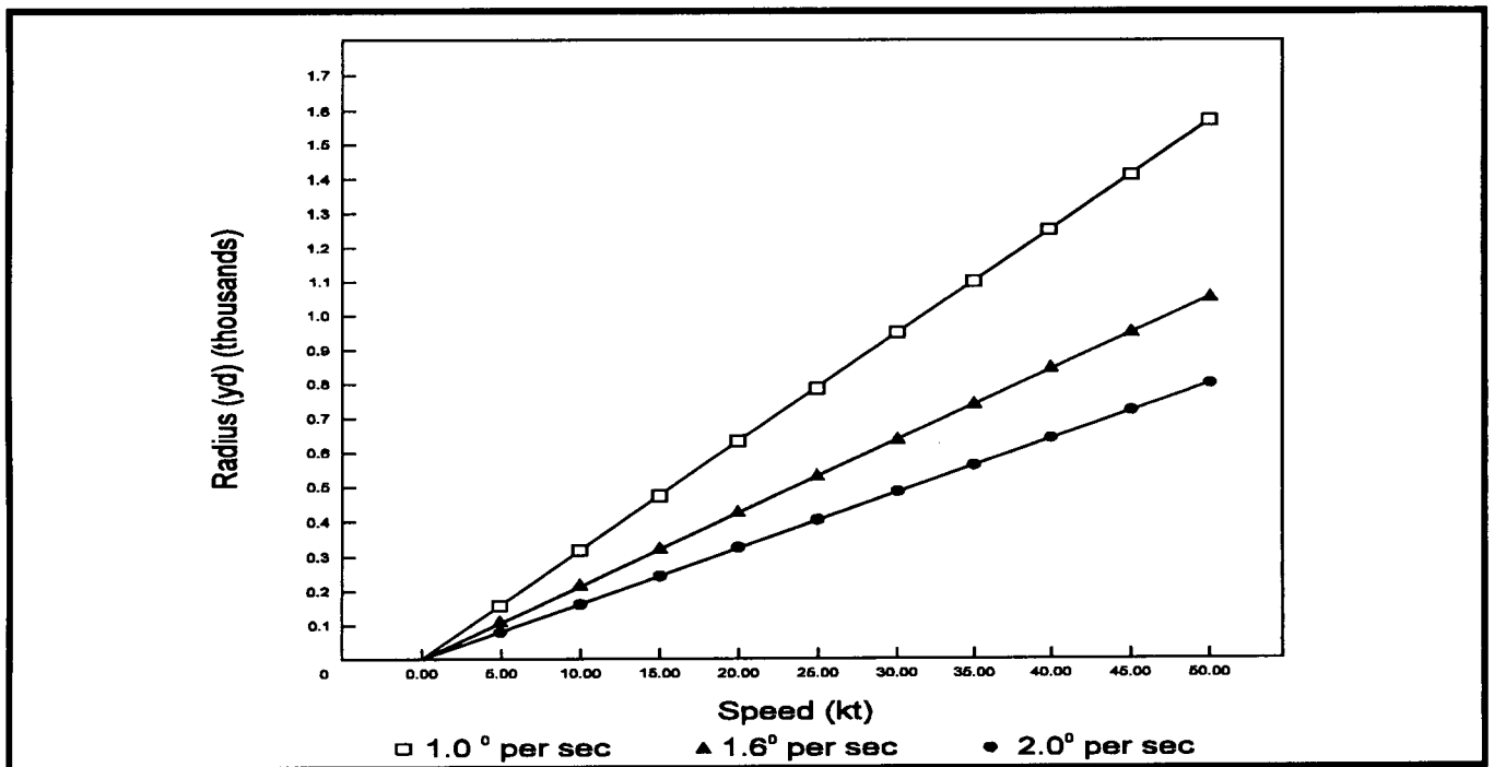
Figure 4-12. Estimated Turn Radii for Various Turn Rates (Sideslip Neglected)
