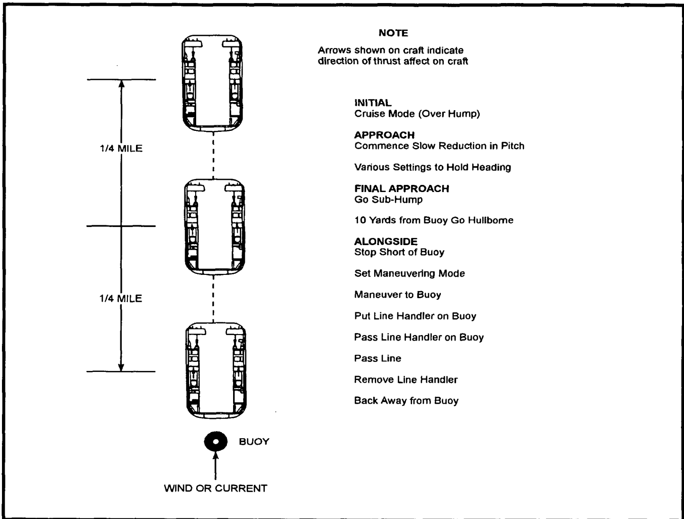
Figure A-10. LCAC Mooring to a Buoy
