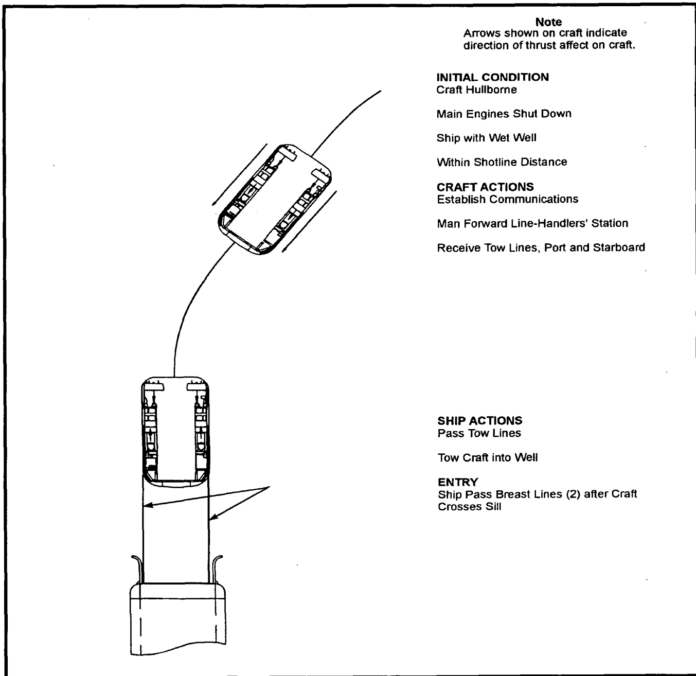
Figure A-6. LCAC Emergency Well Deck Recovery
