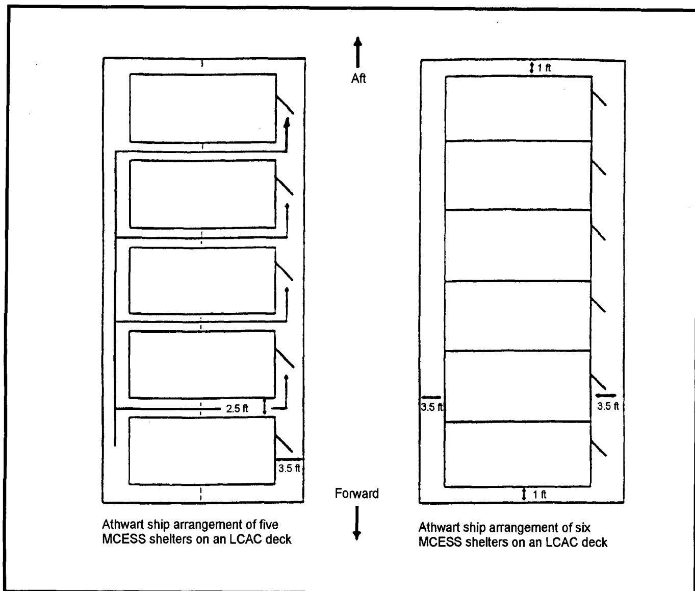
Figure 7-4. MCESS Shelter Configurations (Sheet 2 of 3)
