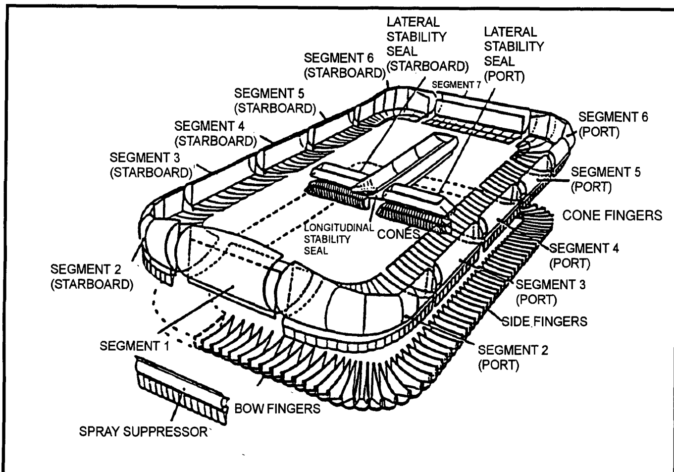
Figure A-2. 3-Dimensional LCAC Skirt Component Drawing
