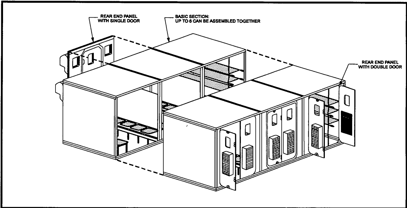
Figure 7-6. PTM-Configured LCAC Assembly
