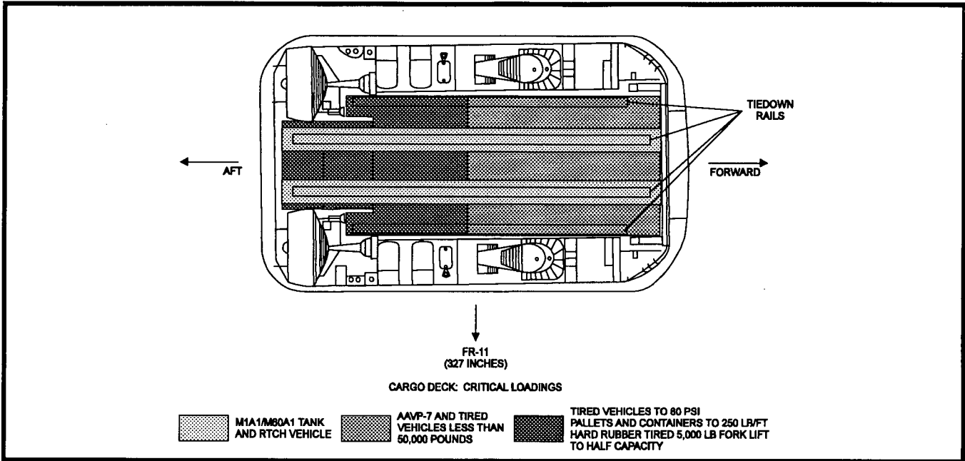
Figure C-1. LCAC Deck Load Diagram
