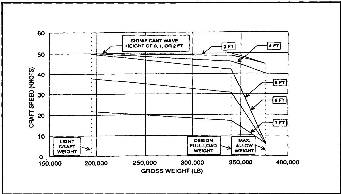
Figure 1-6. Maximum Allowable Speed to Avoid Structural Damage
