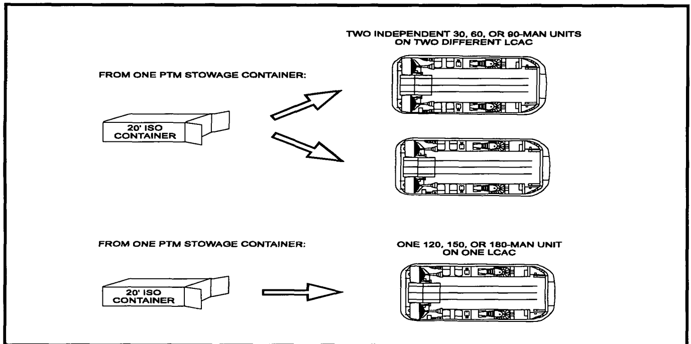
Figure 7-8. PTM-Configured LCAC
